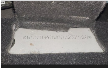
CHASSI
